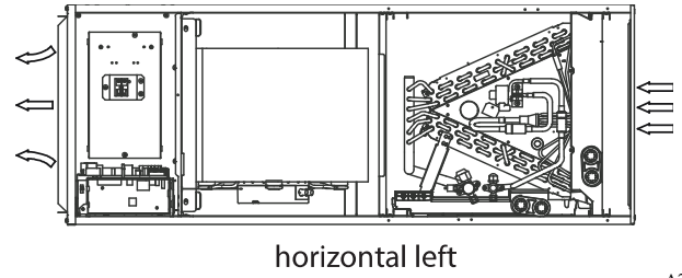
Fig. 7 — Horizontal Left installation
