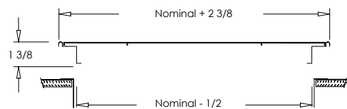
EAD-CAR1-Louver
