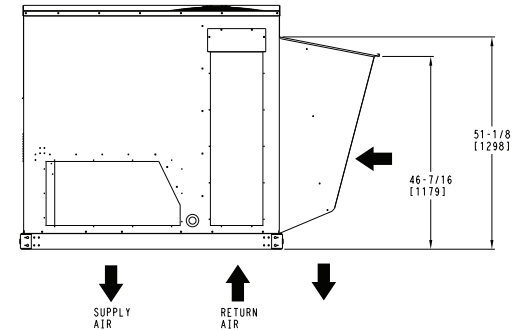
HORIZONTAL ECONOMIZER
