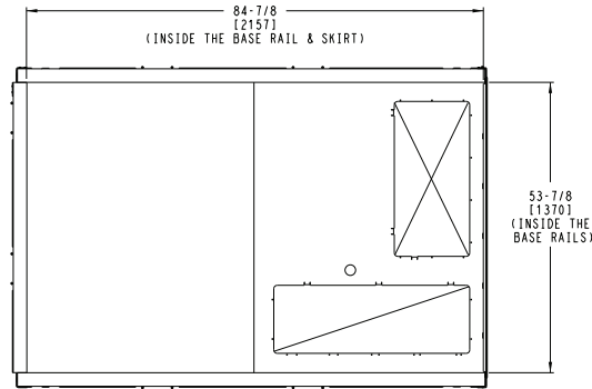
INSIDE BASERAIL DIMENSIONS BOTTOM
