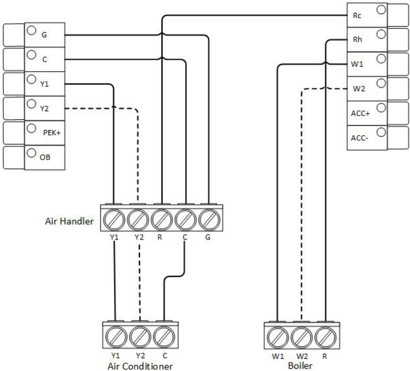
Diagram 10. Two-transformer configuration (Forced-Air Cooling & Radiant Heating)
