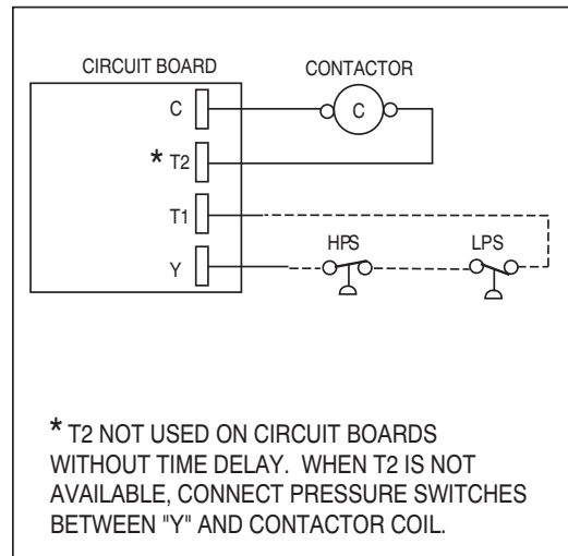
Fig. 4 - Heat Pump Electrical Connections
