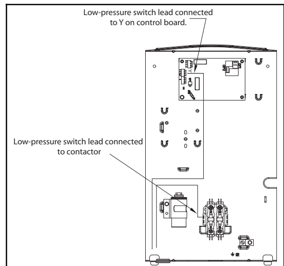
Fig. 5 - Heat Pump Electrical Connections
