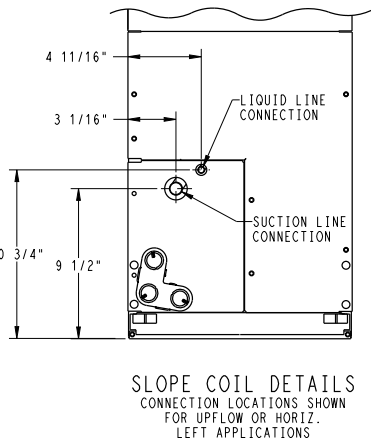
Fig. 1 – Dimensions, sheet 1
