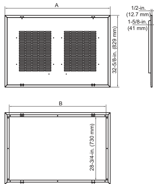
Fig. 1 – Louvered Panel Dimensions
