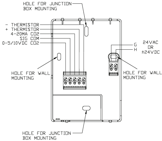
Fig. 3 — CO 2 Sensor 33ZCSPTCO2-01, 33XCSPTCO2LCD-01 — Wiring Diagram
