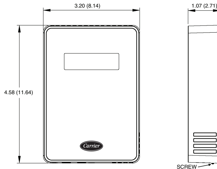
Fig. 1 — CO 2 Sensor (Part No. 33ZCSPTCO2LCD-01) and Dimensions
