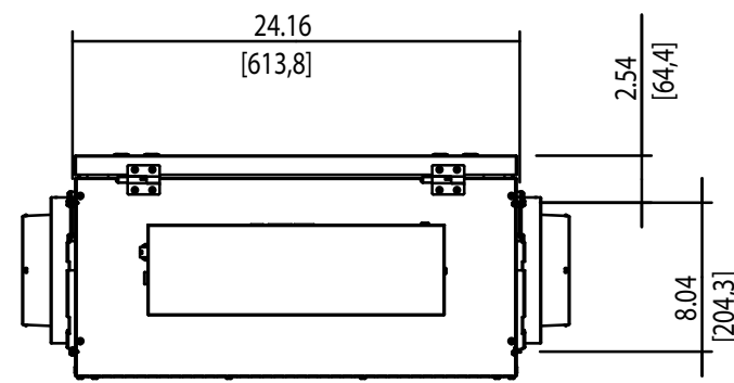
(Ceiling Chain) Hanging Hole Pattern Top View
