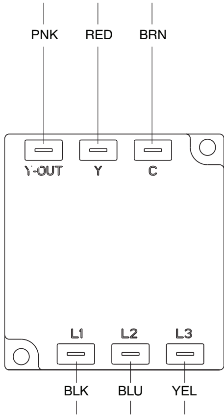
Fig. 5 - Phase Monitor Module Detail (575V)
