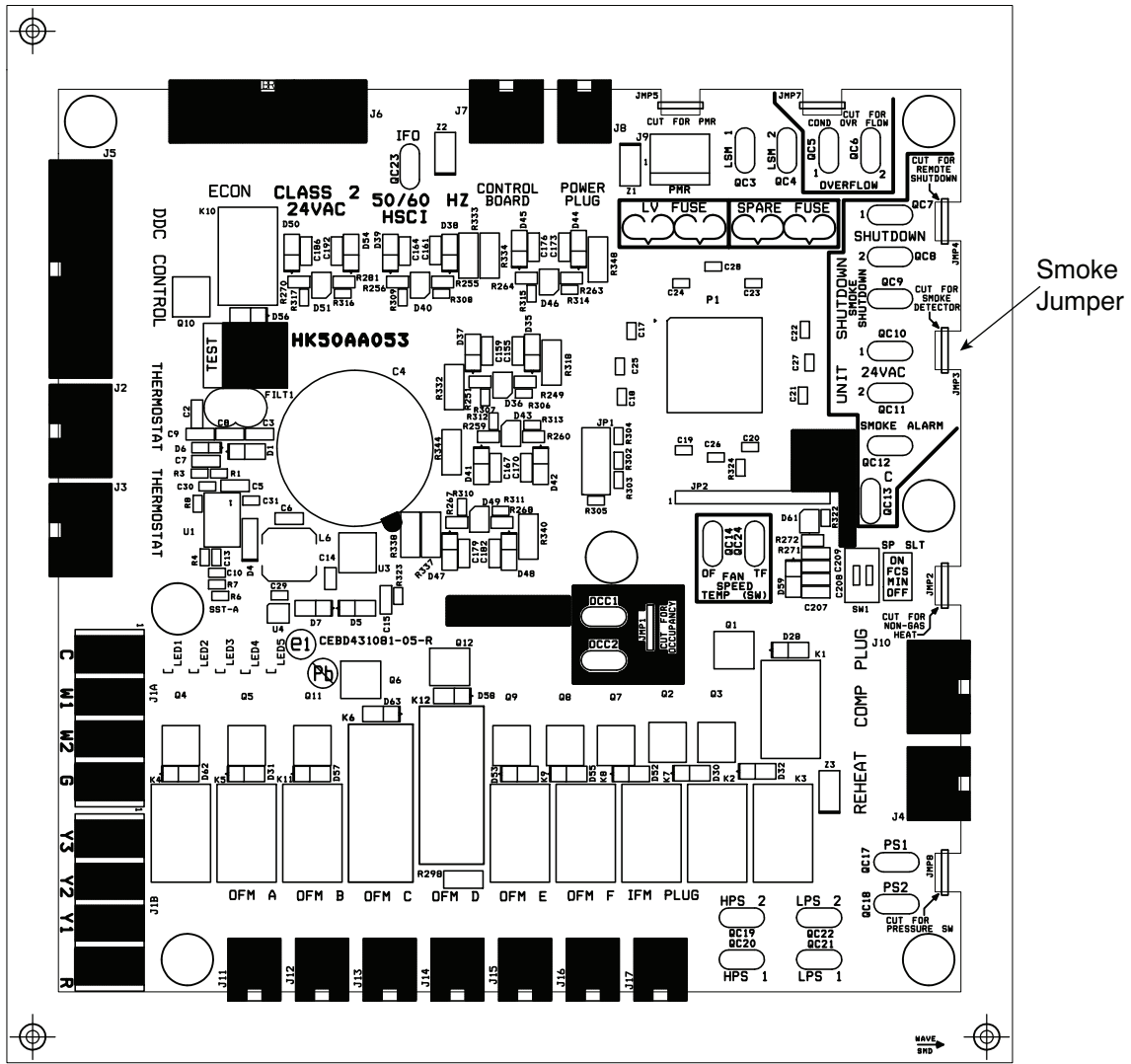
Fig. 3 - 48/50LC Control Board
