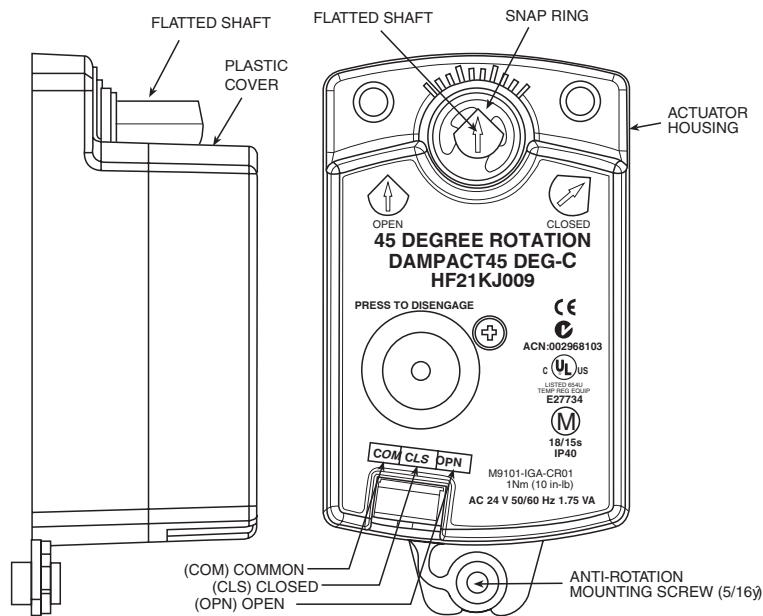
Fig. 2-Actuator Detail (45° round shown)
