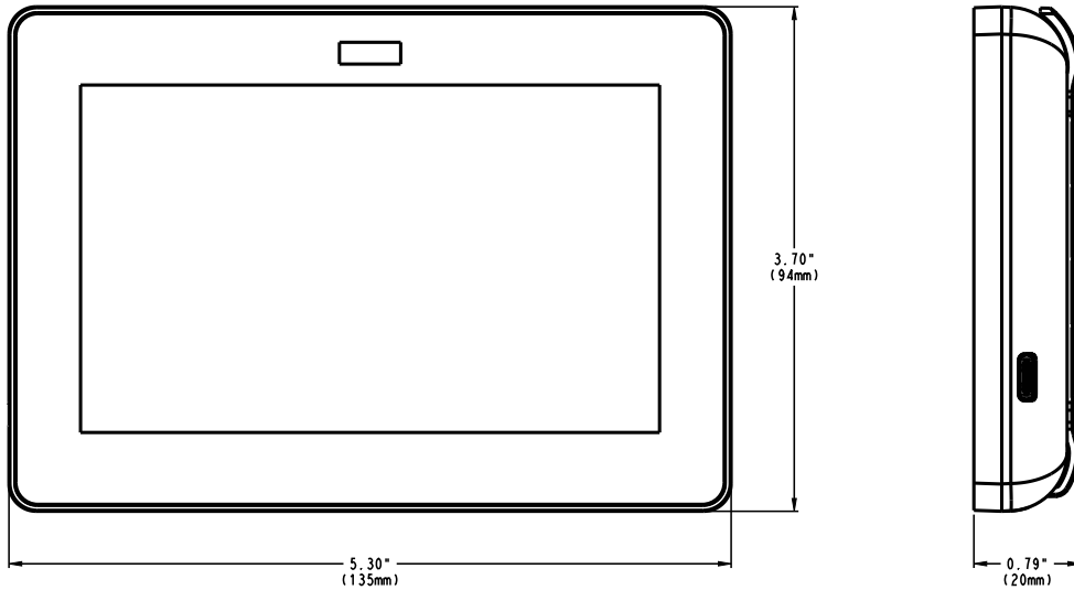
Fig. 1 – Unit Dimensions
