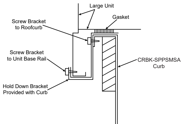
Fig. 6 - Bracket Attachment
