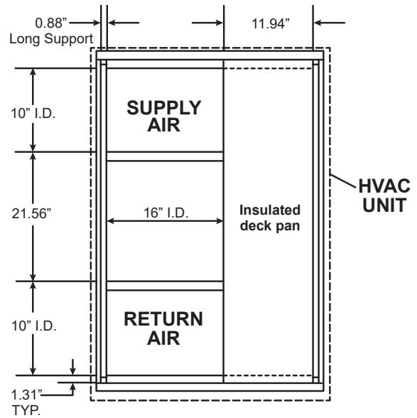
Fig. 3 - CRBK-SPPSMSA Curb with Small Cabinet
