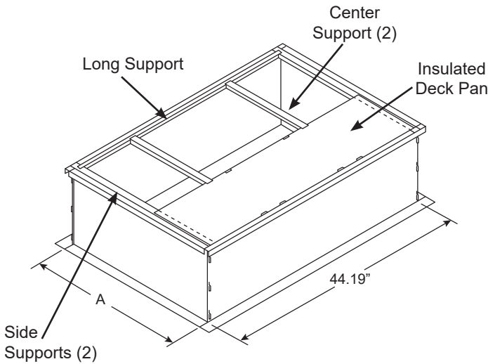
Fig. 2 - Roof Curb Detail (CRBK-SPPSMSA Curb Shown)
