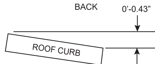
Fig. 7 - Roof Curb Detail
