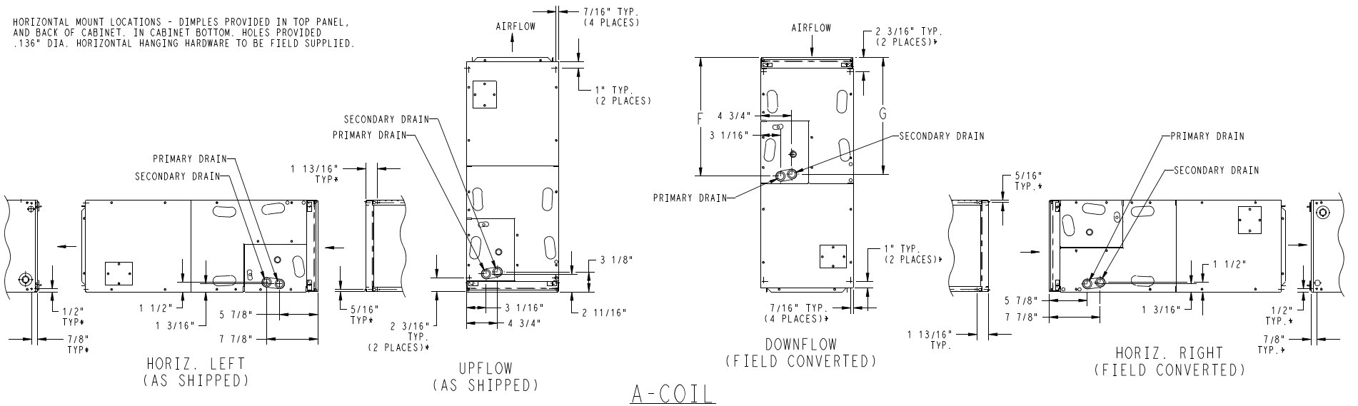
Fig. 2 – F55 Dimensions, English, sheet 2
