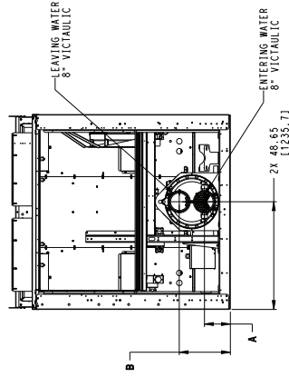
BRINE EVAPORATOR (72" IN MODEL NUMBER POSITION 12)
