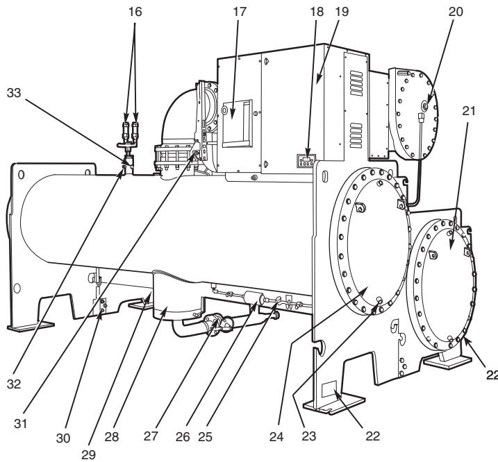
REAR VIEW
