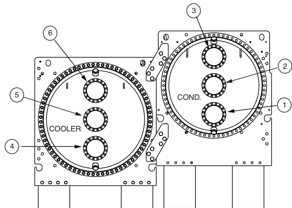
COMPRESSOR END
