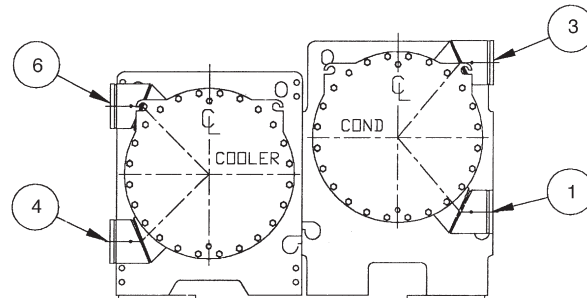
COMPRESSOR END
