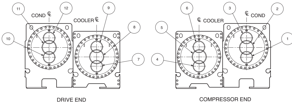
FRAMES 4, 5, AND 6
