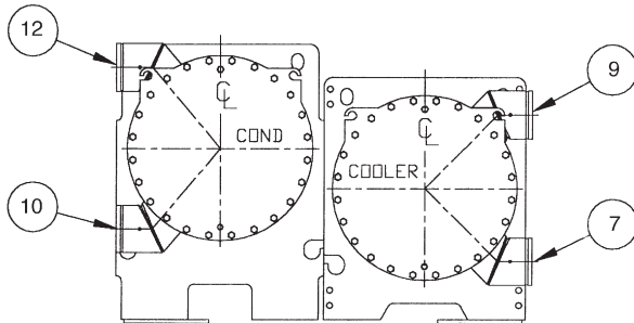
DRIVE END
