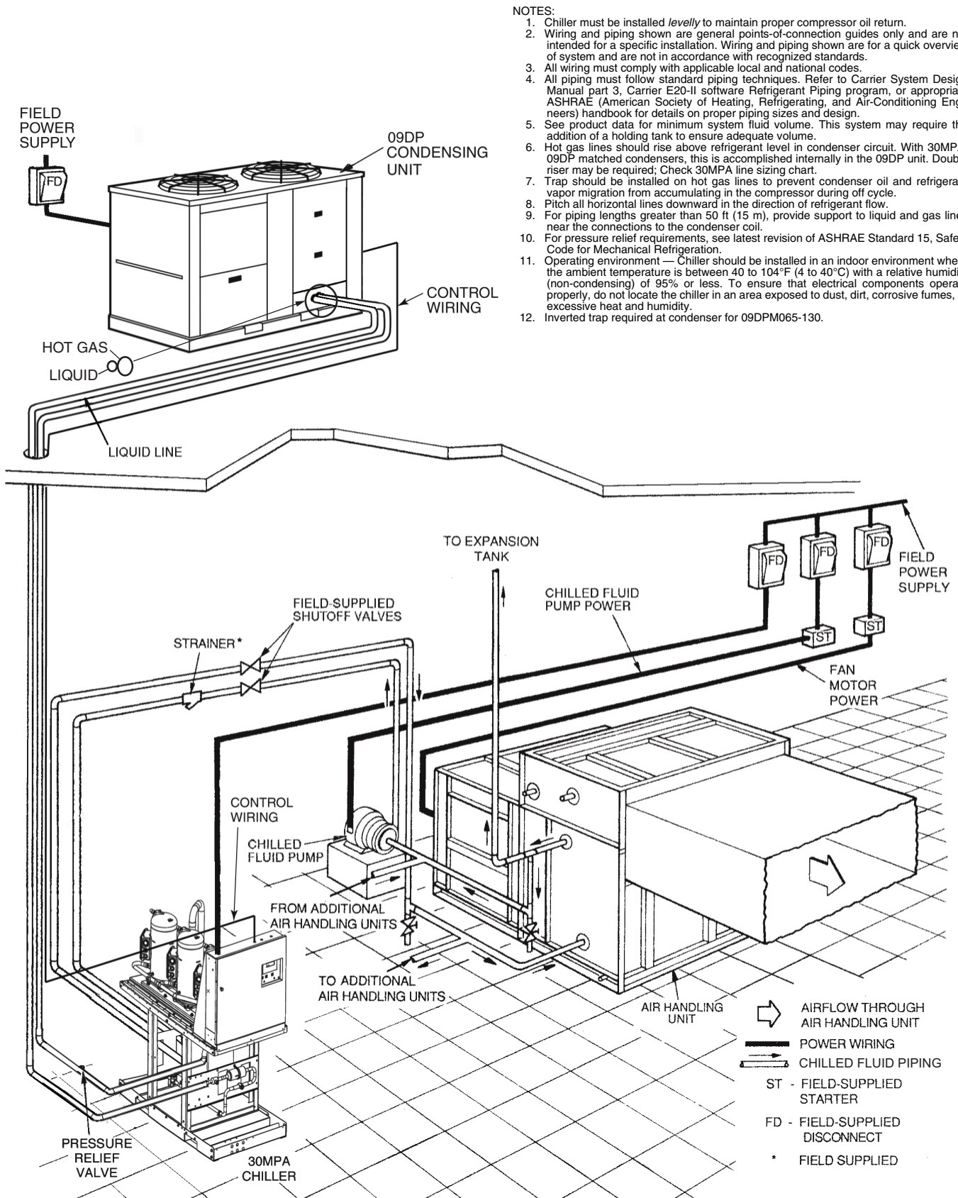
Fig. 26 — Typical Piping and Wiring, 30MPA Unit with 09DP Remote Air-Cooled Condenser Shown
