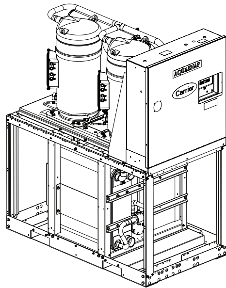
30MPW050-071
