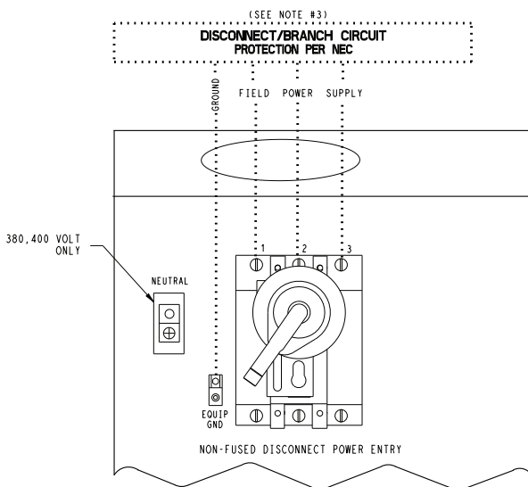
NON-FUSED DISCONNECT
