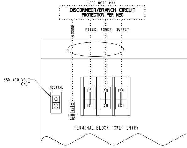
TERMINAL BLOCK
