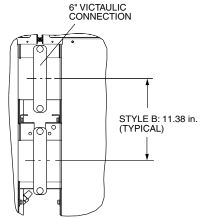
DETAIL A (CORNER POSTS REMOVED FOR CLARITY)
