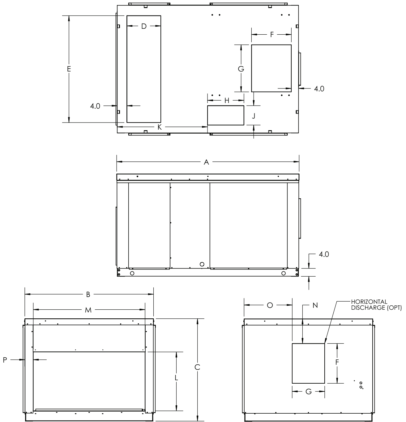
DIMENSIONS (in.)
