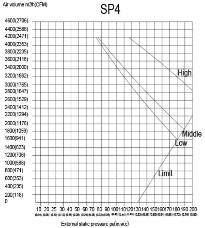
Fig. 19 – Fan Performance – 40MBDQ58
