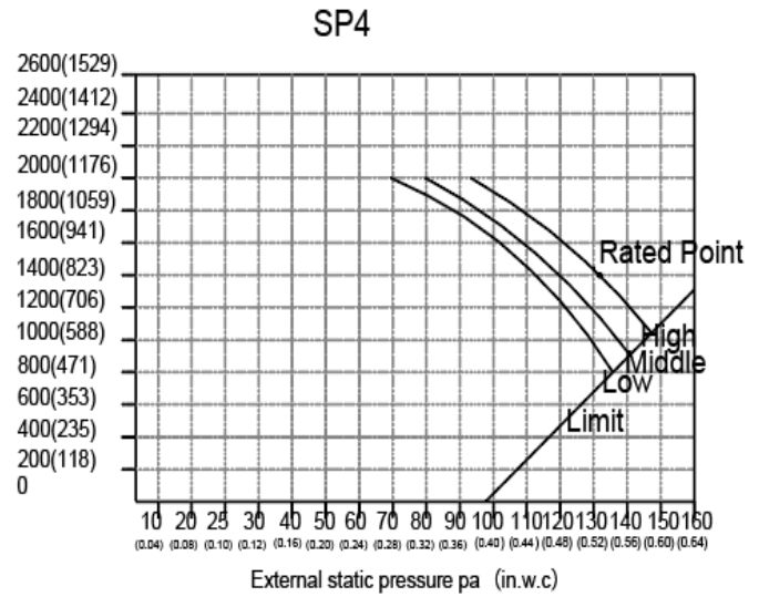
Fig. 18 – Fan Performance – 40MBDQ48
