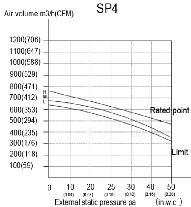
Fig. 13 – Fan Performance – 40MBDQ09
