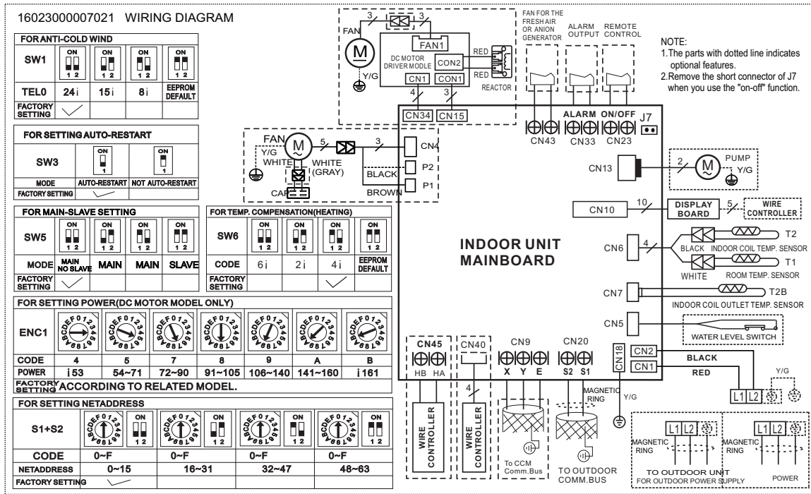
Fig. 22 – Wiring Diagram Size 58
