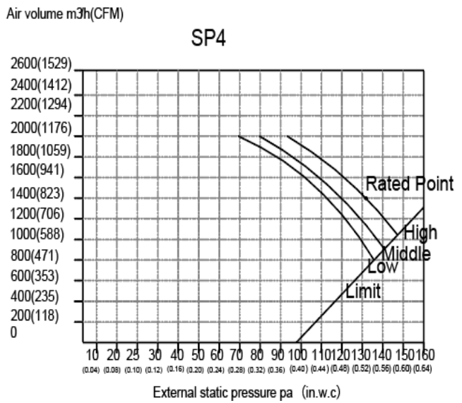
Fig. 16 – Fan Performance – 40MBDQ24
