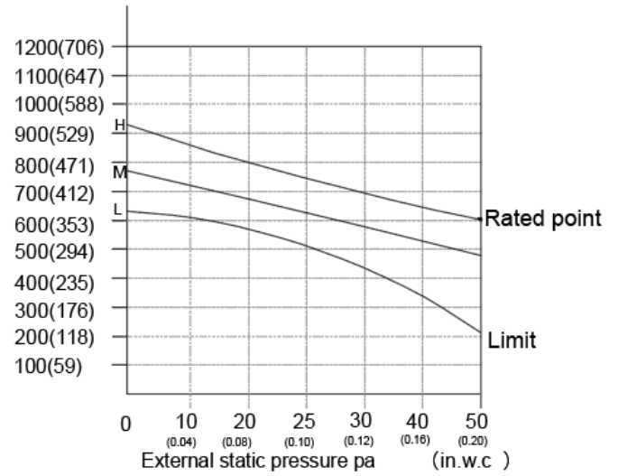
Fig. 14 – Fan Performance – 40MBDQ12
