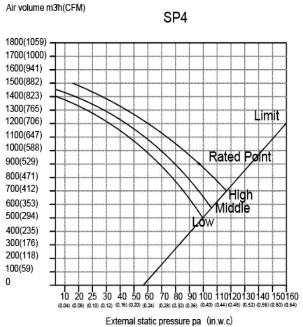
Fig. 15 – Fan Performance – 40MBDQ18
