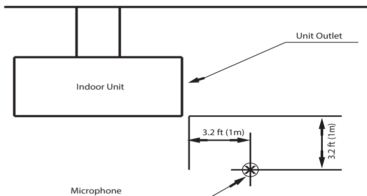
Fig. 10 – Sound Pressure Testing Method
