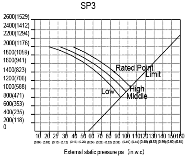
Fig. 18 – Fan Performance – 40MBDQ48
