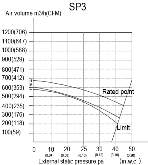
Fig. 13 – Fan Performance – 40MBDQ09
