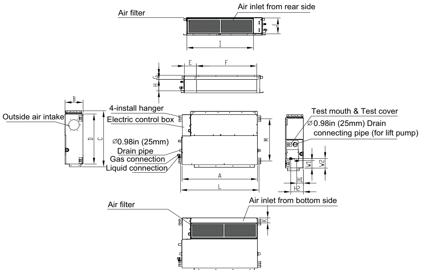
Fig. 3 – Indoor Unit Sizes 9K – 48K
