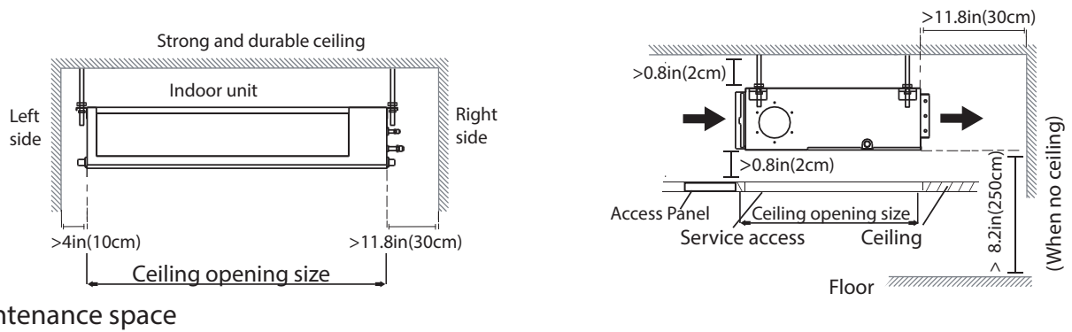
Fig. 5 – Installation Clearances
