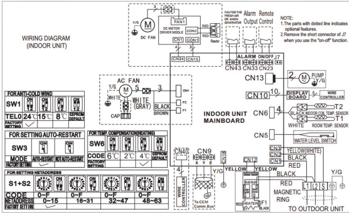
Fig. 20 – Wiring Diagram Size 9K – 24K
