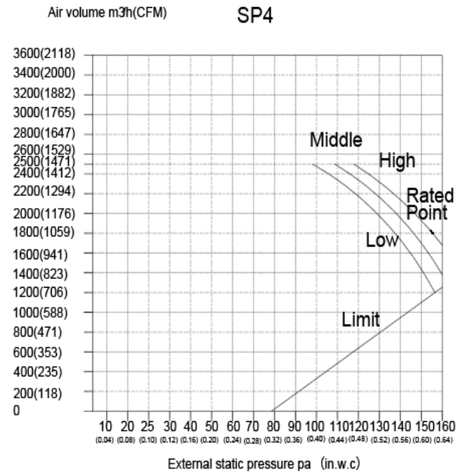
Fig. 17 – Fan Performance – 40MBDQ36
