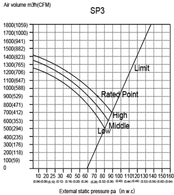
Fig. 15 – Fan Performance – 40MBDQ18
