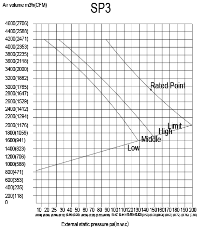
Fig. 19 – Fan Performance – 40MBDQ58
