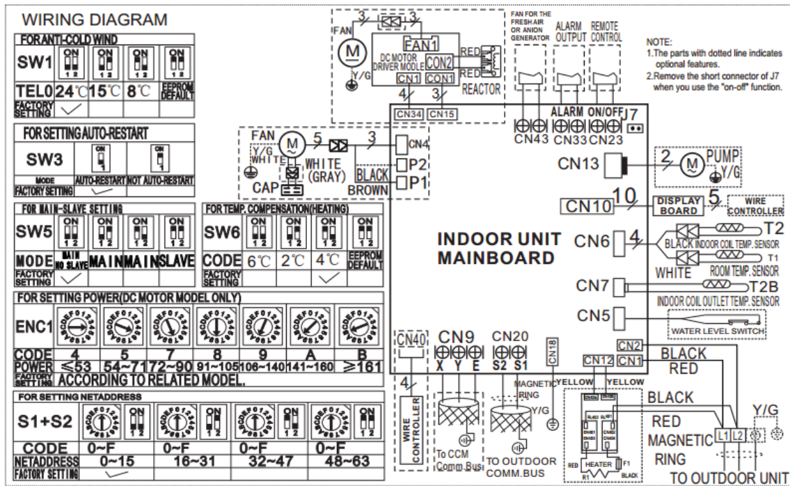
Fig. 21 – Wiring Diagram Size 36K–48K
