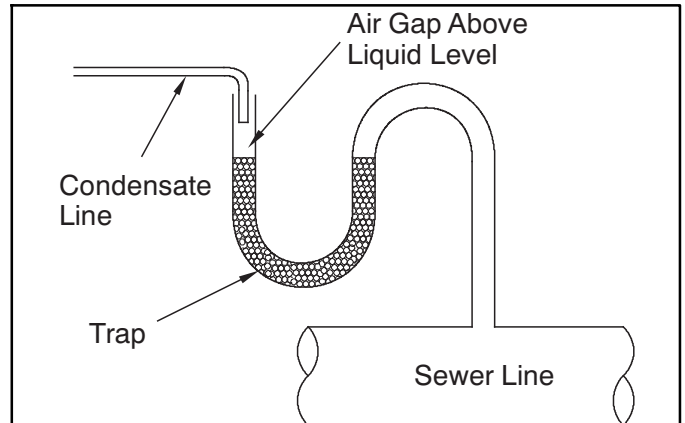
Figure 12 - Condensate Drain to Waste Line
