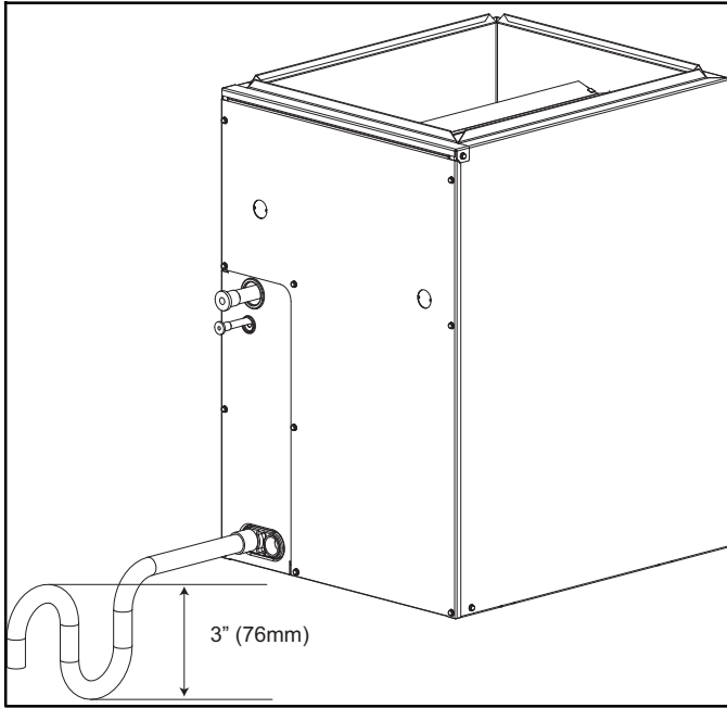
Figure 11 - Condensate Trap
