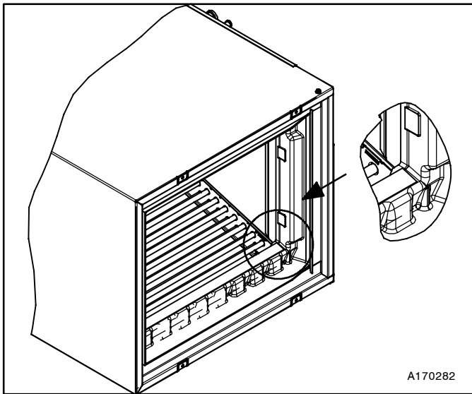
Figure 7 - Condensate Pan Extension Cork Tape Location
