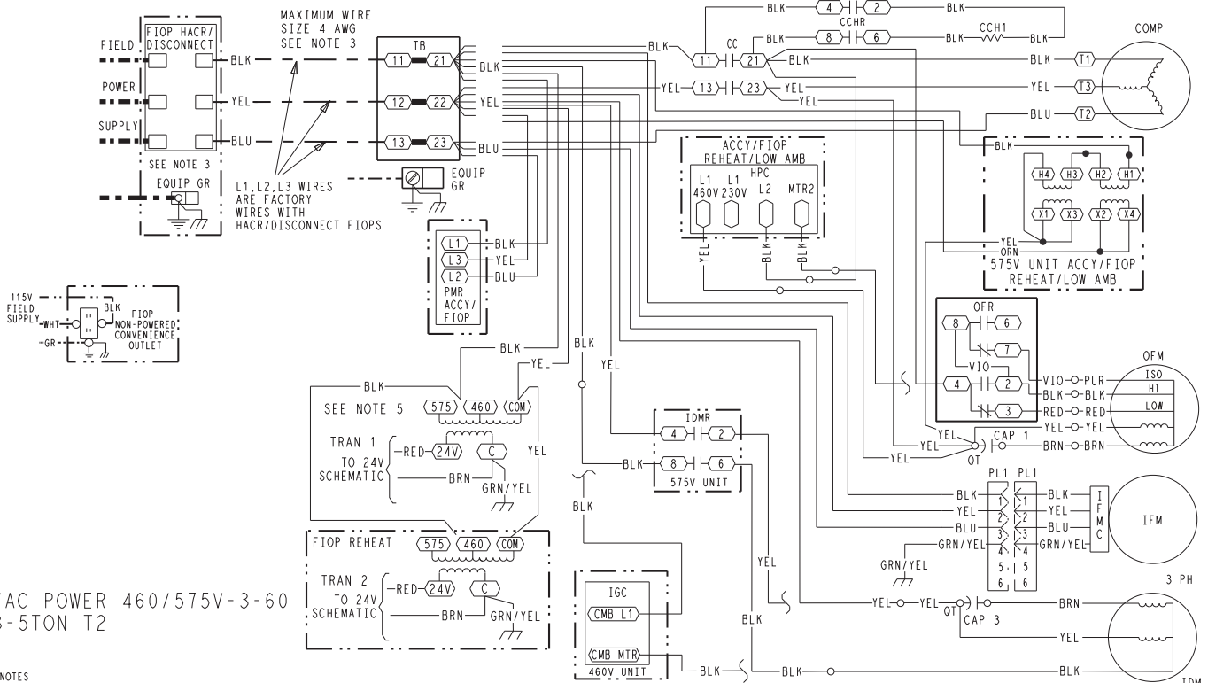
TYPICAL 48GC 04-06 POWER WIRING DIAGRAM, 460-575/3/60 UNIT SHOWN
