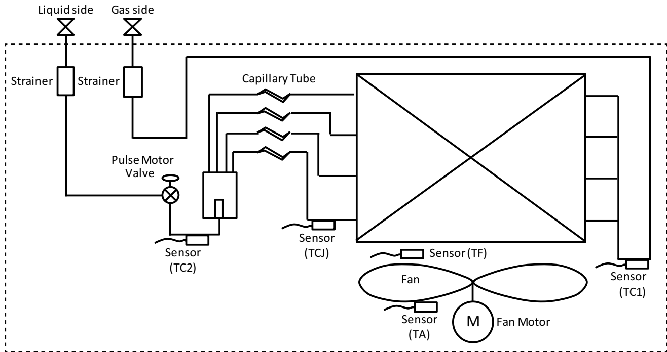
Fig. 8 —Piping
