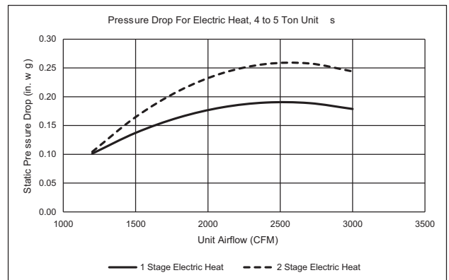
Fig. 16 —Pressure Drop for Electric Heat 4 to 5 Ton Units - 1 and 2 - Stage Heat
