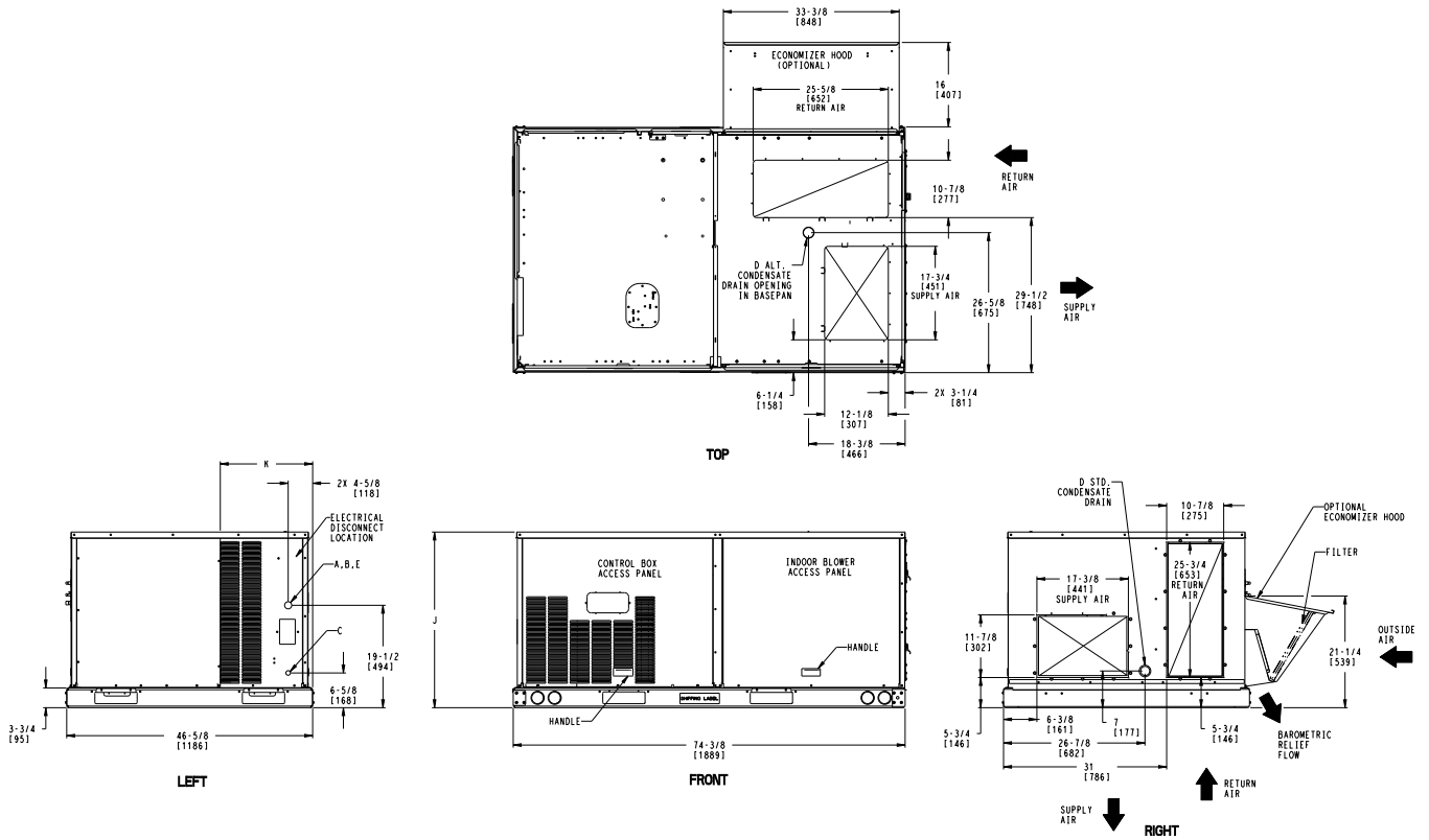
Fig. 3 — Dimensional Drawing
