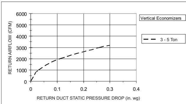
Fig. 13 —Return Air Pressure Drop- Vertical 3- 5 Ton
