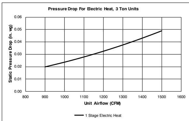
Fig. 15 —Pressure Drop for Electric Heat 3 Ton Units - 1-Stage Unit
