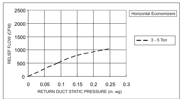
Fig. 12 —Barometric Relief Flow - Horizontal 3- 5 Ton
