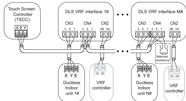
Fig. 5 —Communication Wiring
