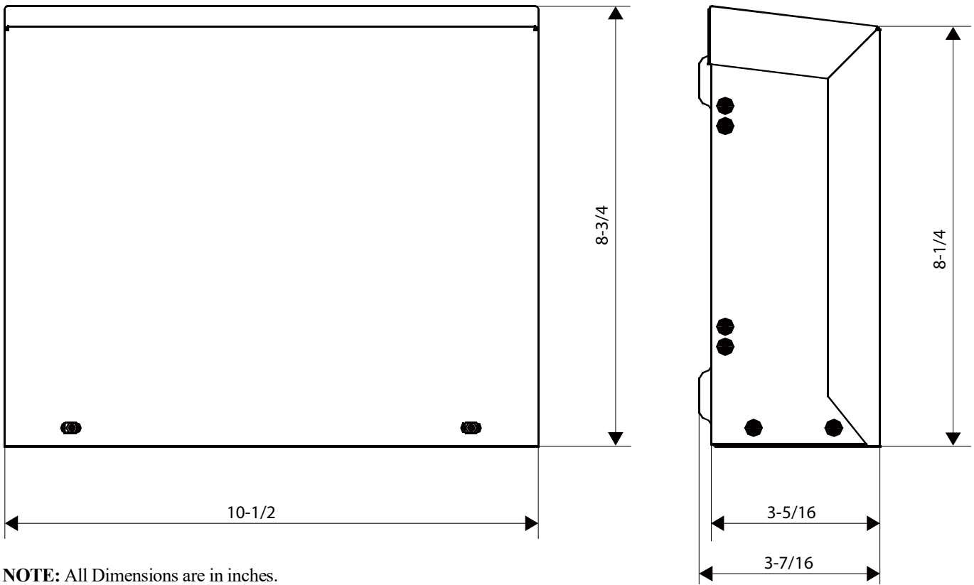
Fig. 1 —Dimensional Drawing
