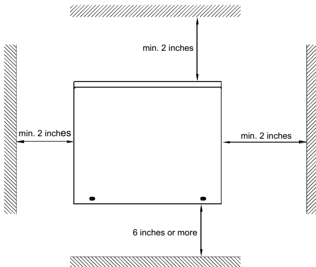
Fig. 2 —Mounting Clearances
