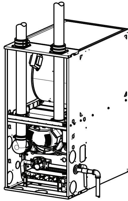
Fig. 9 - Assembled View of Internal Vent Kit
