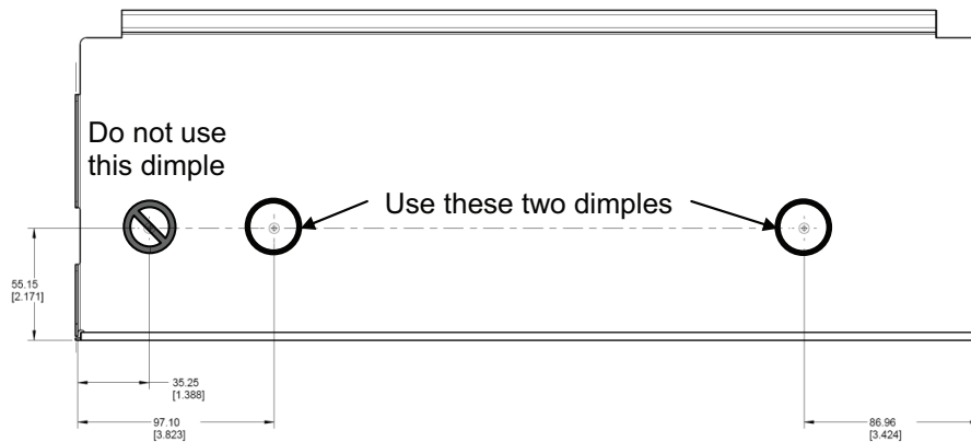
Fig. 2 - Bottom Plate Dimple Location
