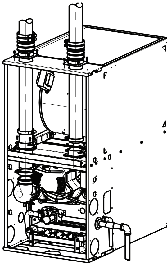
Fig. 11 - Exploded View of Internal Vent Kit
