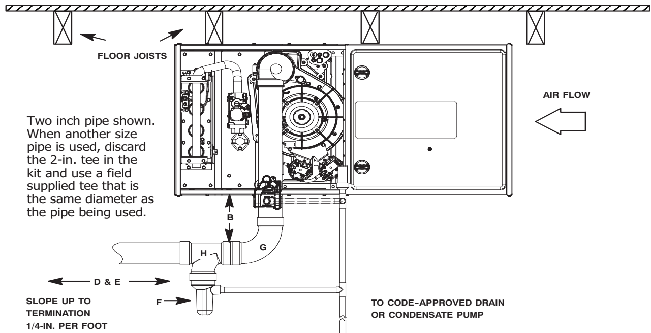
CONFIGURATION FOR VENT AND/OR COMBUSTION AIR PIPING (See NOTES in Figure 1)
