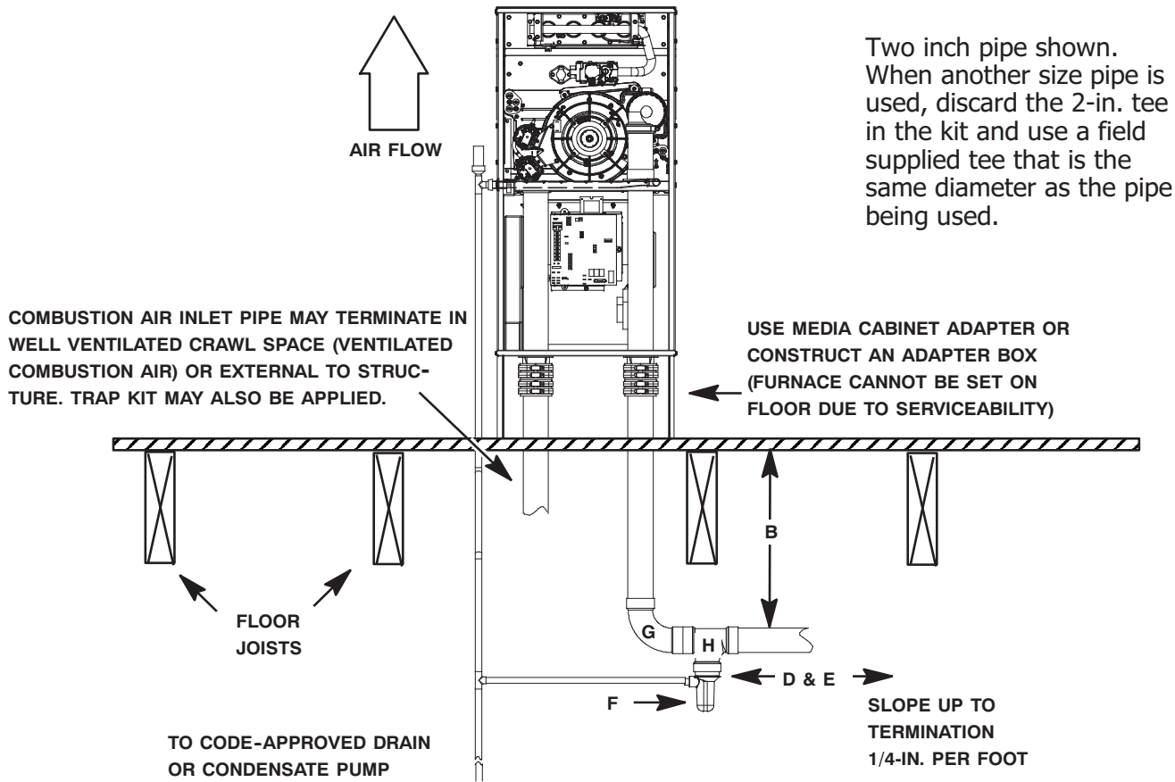
CONFIGURATION FOR VENT AND/OR COMBUSTION AIR PIPING (See NOTES in Figure 1)
