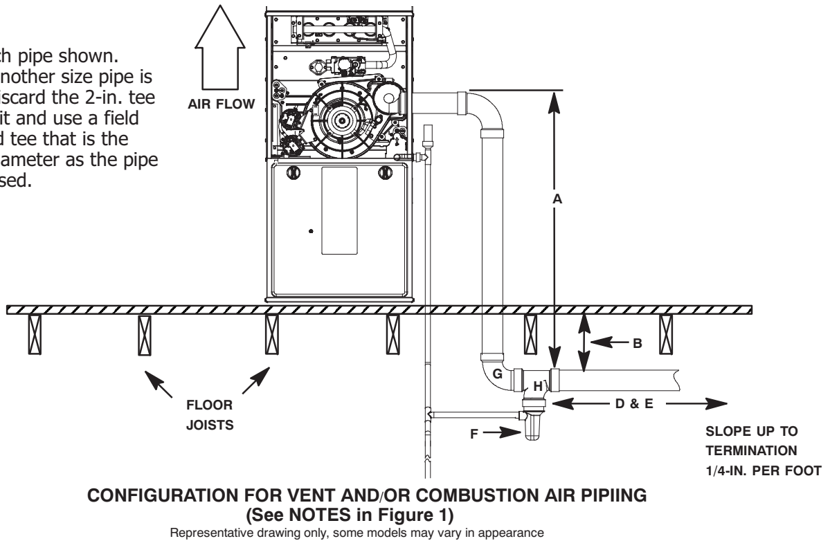
Fig. 6 – Vent Located Below Floor with Upflow Furnace and Side Venting
