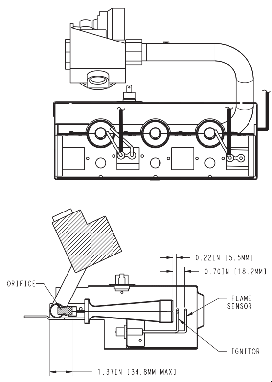
Fig. 3 - Single-Stage Igniter, Flame Sensor, Orifice/Main Burner Relationship
