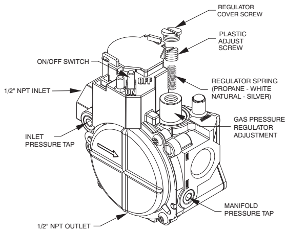
Fig. 4 - Single-Stage Gas Valve
