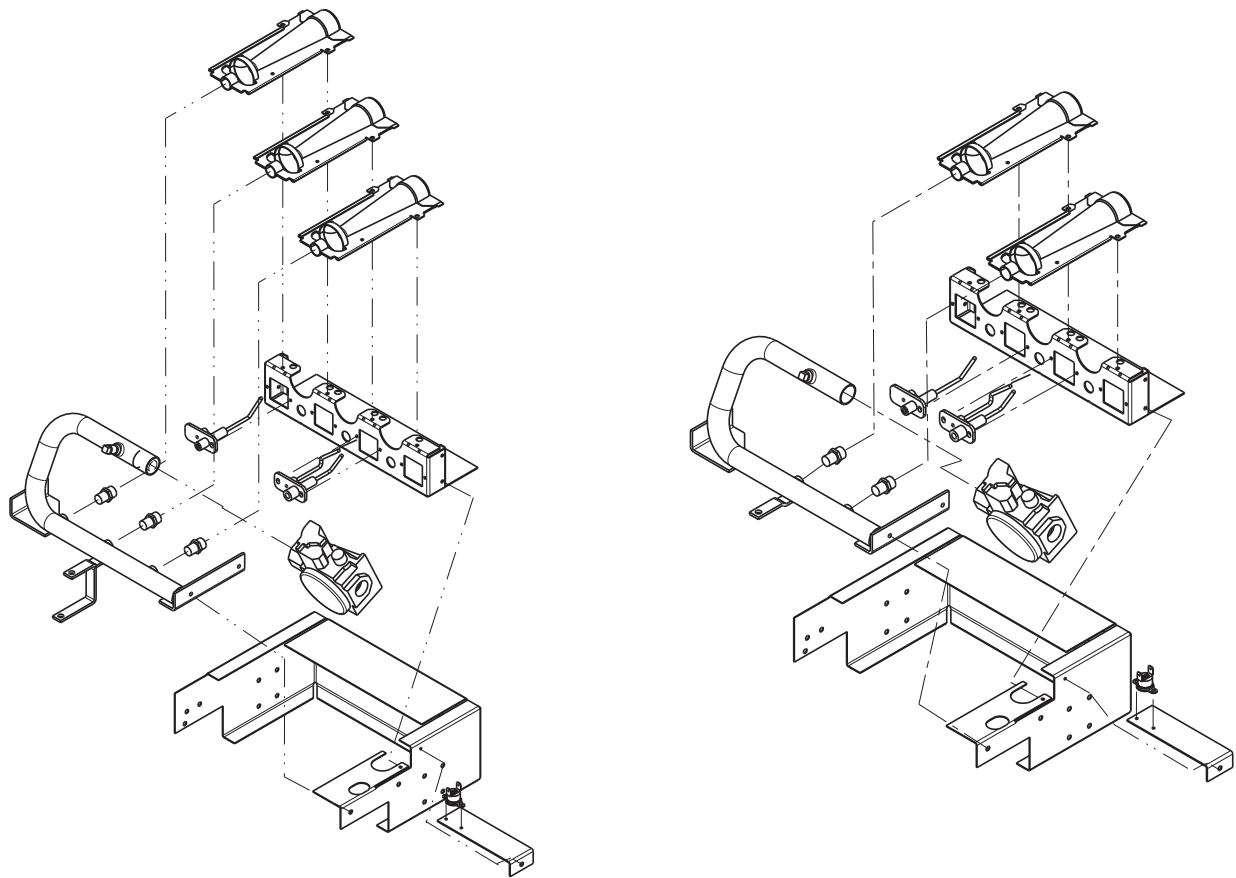
Fig. 4 - Single-Stage Gas Valve
