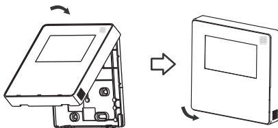
Fig. 8 — Reattaching the Front Cover of the Wired Controller
