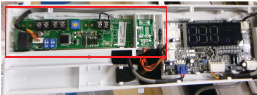
Fig. 13 — Install the multifunction board
