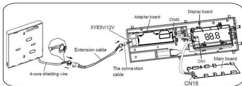
Fig. 9 — Installation of KSACN0801AAA
