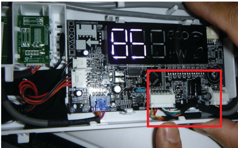
Fig. 16 — Connect the new 7-pin plug
