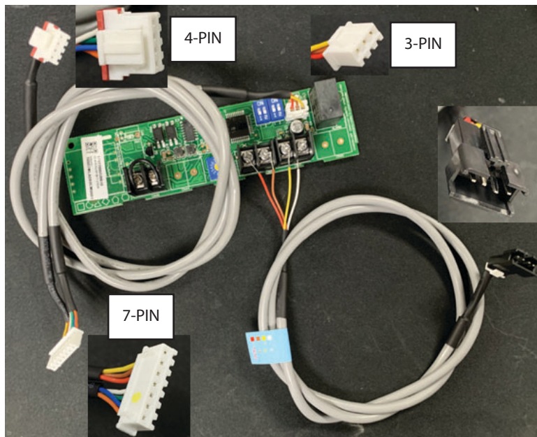
Fig. 15 — Identify the connections
