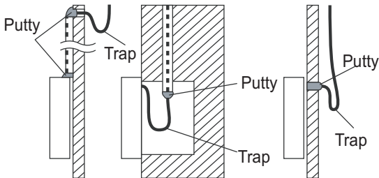
Fig. 7 — Seal the wires
