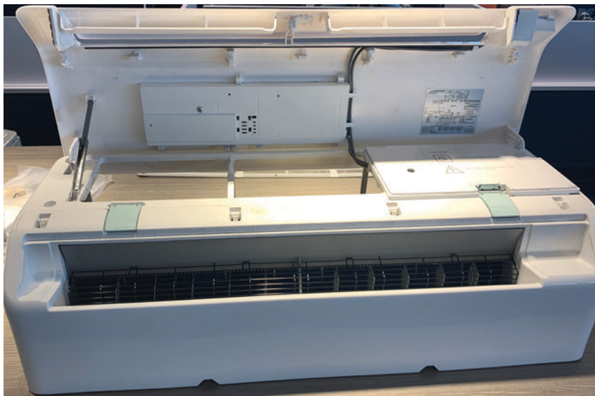
Fig. 11 — Open the front panel
