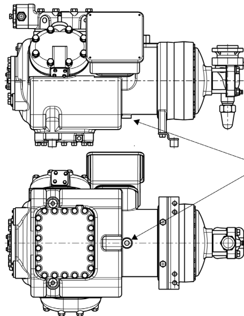
Fig. 11 — 06E Motor Barrel Equalization Port
