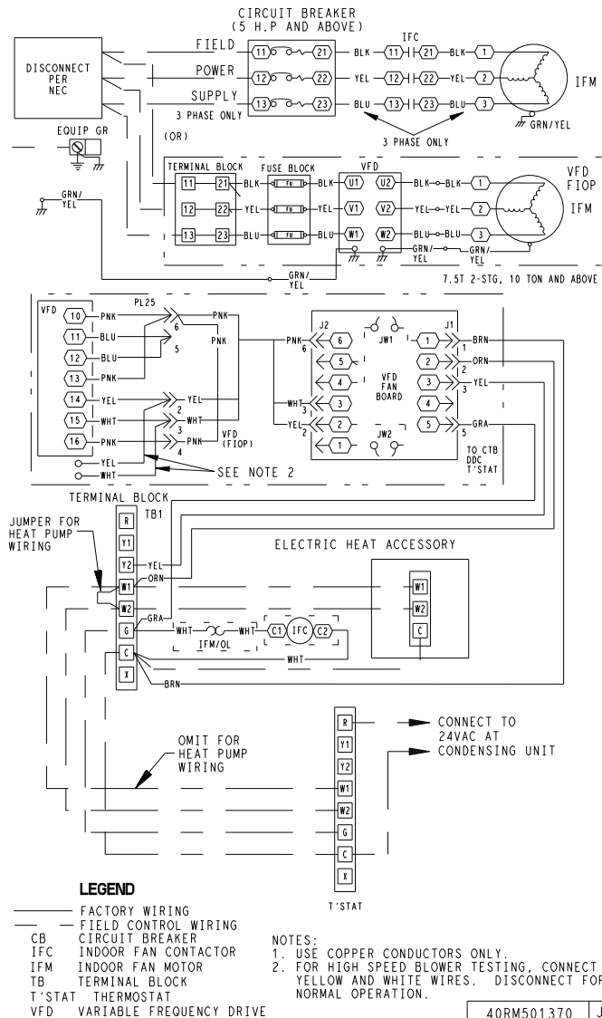
Fig. 37 — Typical Wiring Diagram — Split System Air-Handling Unit (524J with ACH550 VFD shown)
