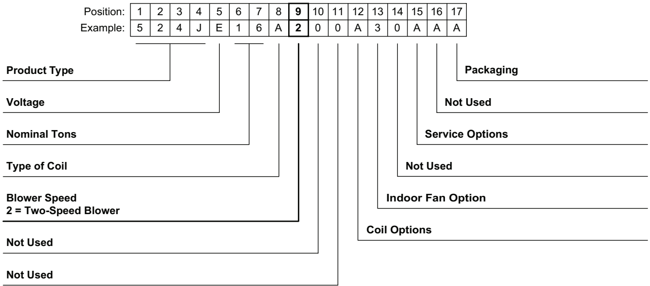
Fig. 4 — Model Number Nomenclature Example, 524J-Series
