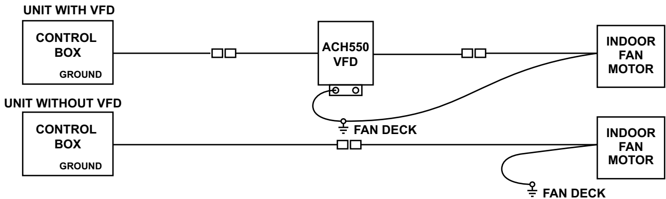
Fig. 42 — To Bypass the VFD on 580J/558J 16-30, 548J 14-24, and 581J/551J 17-28 Units
