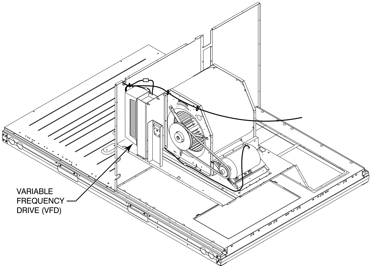
Fig. 9 — ACH550 VFD Location for the following units: 581J/551J 07 and 549J 07
