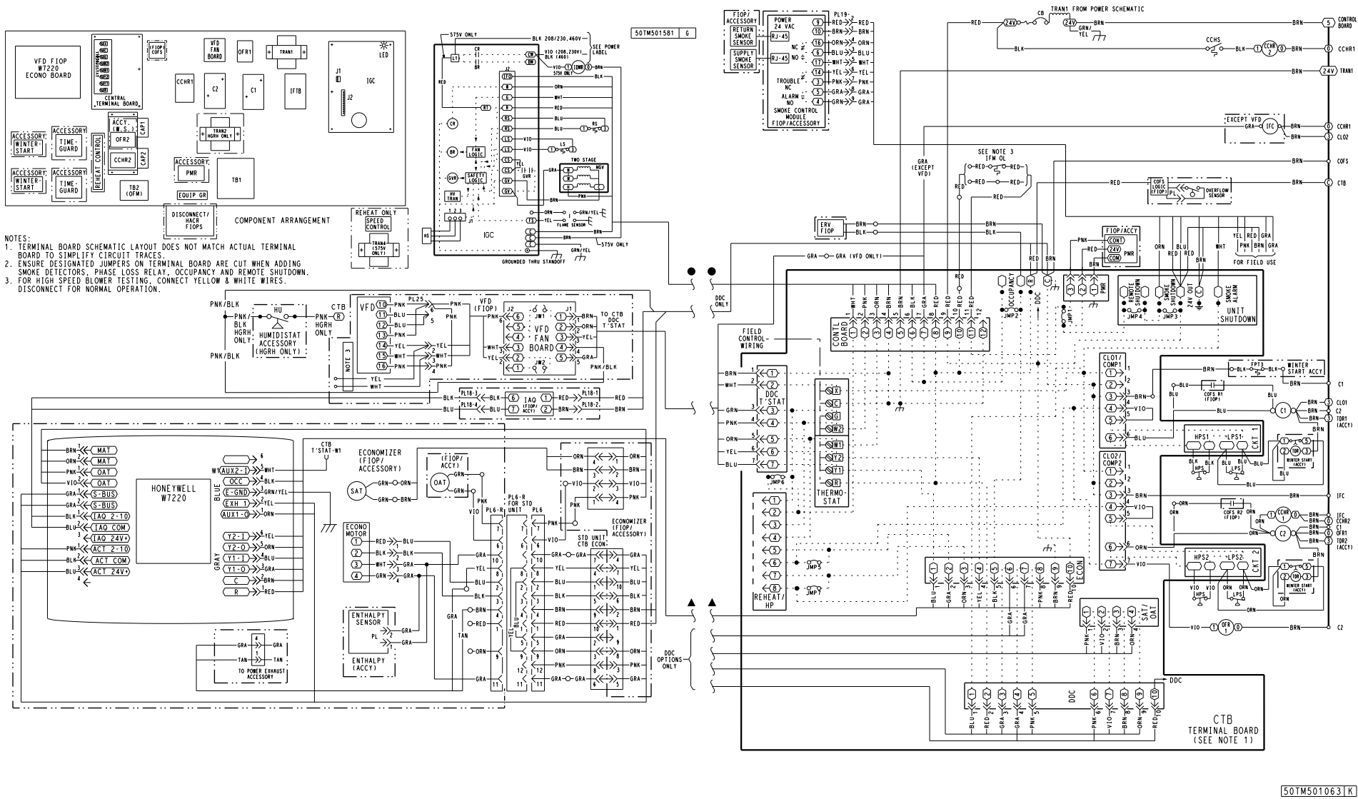
Fig. 33 — Typical Wiring Diagram — Single Package Rooftop Unit (581J*14 with ACH550 VFD shown)
